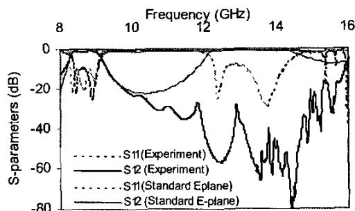
Figure 3: Measured response of the fabricated prototype (dimensions as in Table 1)
